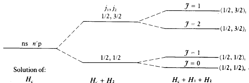
7.9 The splitting of levels in j - j coupling.
